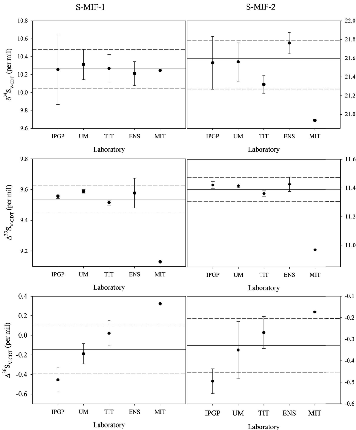
Fig. 1 The individual laboratory results of S-MIF-1 and S-MIF-2. The error bars for the individual laboratory results are 1 \sigma ; the solid and dashed lines represent the interlaboratory averages and \pm 1\sigma , respectively.
