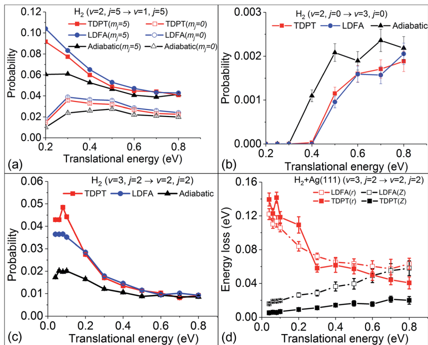
Fig. 5 (a) Vibrational state-to-state deexcitation probabilities from H 2 ( \nu = 2, j = 5 ) to H 2 ( \nu = 1, j = 5 ) for rotationally excited initial conditions as predicted with MD, MDEF(LDFA), and MDEF(TDPT). (b) Vibrational excitation probabilities upon scattering. (c) Vibrational deexcitation probability from H 2 ( \nu = 3, j = 2 ) to H 2 ( \nu = 2, j = 2 ). (d) Energy loss during vibrational deexcitation from H 2 ( \nu = 3, j = 2 ) to H 2 ( \nu = 2, j = 2 ).
