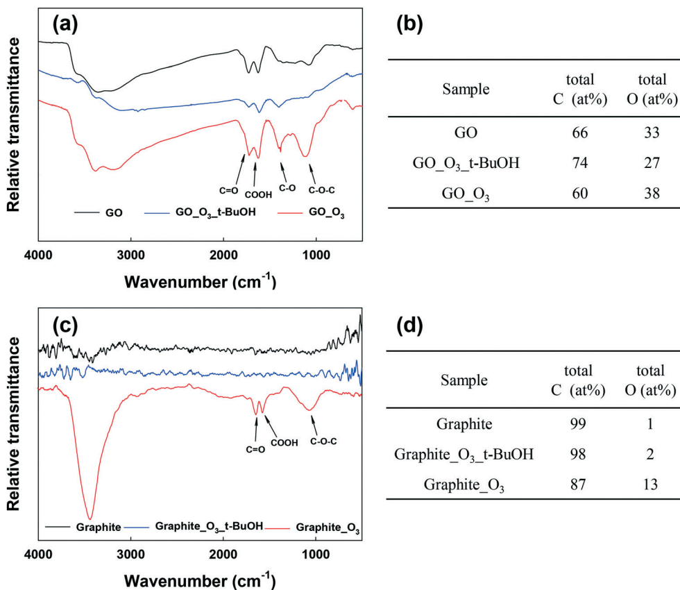
Fig. 4 (a) FTIR spectra of GO, GO- \text{O}_3 with t-BuOH and GO- \text{O}_3 . (b) C and O ratio of GO, GO- \text{O}_3 and GO- \text{O}_3 with t-BuOH obtained from XPS analysis. (c) FTIR spectra of graphite, Graphite- \text{O}_3 with t-BuOH and Graphite- \text{O}_3 . (d) C and O ratio of graphite, Graphite- \text{O}_3 and Graphite- \text{O}_3 with t-BuOH obtained from XPS analysis.
