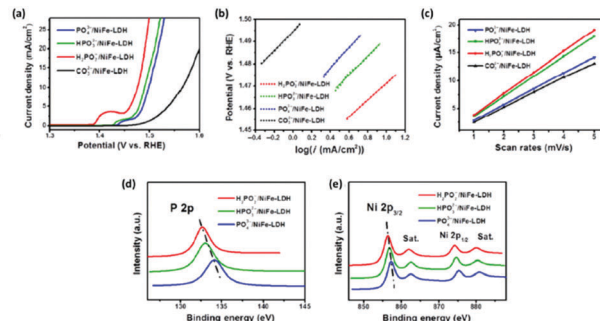
Fig. 12 (a) Polarisation curves of four LDH catalysts ( \text{PO}_4^{3-}/\text{NiFe-LDH} , \text{HPO}_3^{2-}/\text{NiFe-LDH} , \text{H}_2\text{PO}_2^-/\text{NiFe-LDH} , and \text{CO}_3^{2-}/\text{NiFe-LDH} ); \text{H}_2\text{PO}_2^-/\text{NiFe-LDH} shows the lowest onset potential and fastest current density increase; (b) Tafel plots, (c) C_{dl} calculations for the four catalysts. XPS data of the \text{PO}_4^{3-}/\text{NiFe-LDH} , \text{HPO}_3^{2-}/\text{NiFe-LDH} , and \text{H}_2\text{PO}_2^-/\text{NiFe-LDH} : (d) P 2p and (e) Ni 2p spectra. (Adapted with permission (ref. 114) Copyright Springer (2017).)
