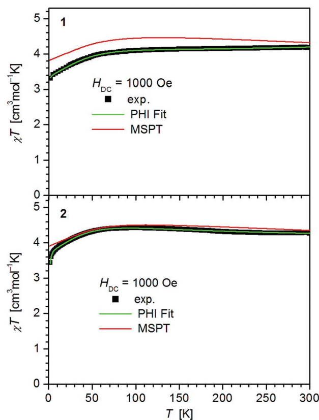
Fig. 2 Temperature dependence of \chi T for 1 and 2. Solid green lines represent the results of the simultaneous fittings with the temperature dependent magnetization (Table 3, Fig. S11†) according to a spin Hamiltonian (eqn (S1)†) by the PHI program. 21 Red lines represent the results of the quantum chemical calculations (MS-CAS(12,13)PT2) (see also Fig. S23†).
