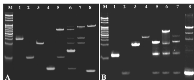
Fig. 1 (A) Lane 1: 1.5 \mu\text{M} walker DNA; lane 2: 4 \mu\text{M} protecting DNA; lane 3: 1.5 \mu\text{M} support DNA ( S_2 ); lane 4: 4 \mu\text{M} target; lane 5: 1.5 \mu\text{M} walker DNA + 4 \mu\text{M} protecting DNA; lane 6: 1.5 \mu\text{M} walker DNA + 4 \mu\text{M} protecting DNA + 1.5 \mu\text{M} support DNA + 4 \mu\text{M} target; lane 7: 1.5 \mu\text{M} walker DNA + 1.5 \mu\text{M} support DNA; and lane 8: 1.5 \mu\text{M} walker DNA + 1.5 \mu\text{M} support DNA + 5 U nicking endonuclease. (B) Lane 1: 1 \mu\text{M} H 1 ; lane 2: 1 \mu\text{M} S 3 ; lane 3: 1 \mu\text{M} H 2 ; lane 4: 1 \mu\text{M} H 3 /S 1 ; lane 5: 1 \mu\text{M} H 1 + 1 \mu\text{M} S 3 ; lane 6: 1 \mu\text{M} H 1 + 1 \mu\text{M} S 3 + 1 \mu\text{M} H 2 ; lane 7: 1 \mu\text{M} H 1 + 1 \mu\text{M} S 3 + 1 \mu\text{M} H 3 /S 1 ; and lane 8: HCR product in the presence of the mixture of H 1 , S 3 , H 2 , and H 3 /S 1 .
