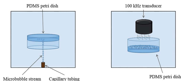
Fig. 1 Design apparatus for controlled cavitation simulation on PDMS films. MBs are initially collected on PDMS films when the Petri dish is directed downward. The Petri dish is then rotated 180^\circ and exposed to an ultrasound transducer that induces dramatic MB oscillation, resulting in cavitation.
