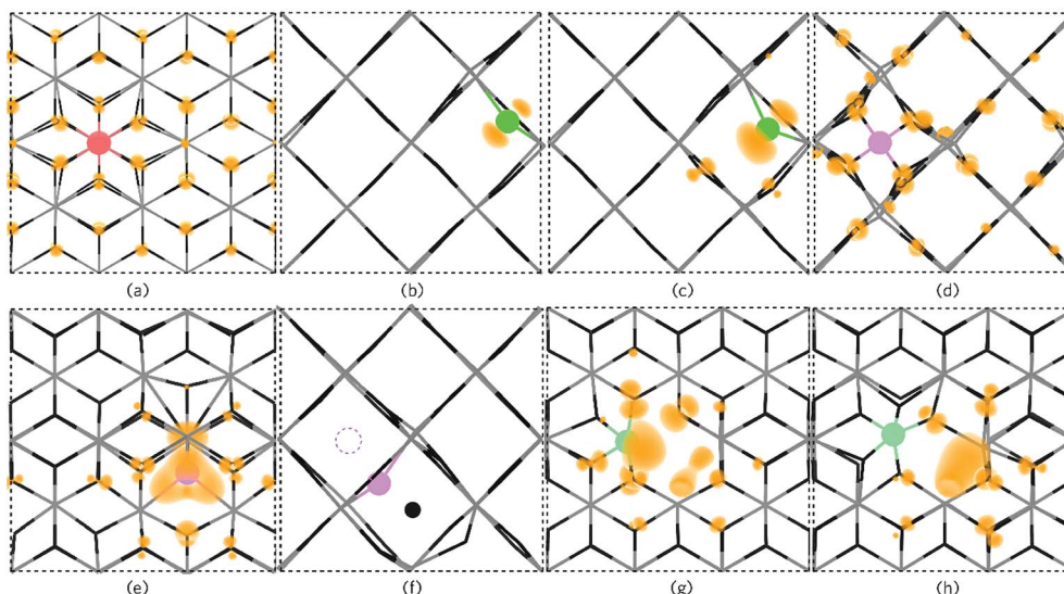
Fig. 7 The partial electron charge densities (orange) for (a) P_{Sn} viewed along \{010\} with a charge density of 0.002 eV \text{ \AA}^{-1} , (b) P_O^0 and (c) P_O^{1-} as viewed along the \{001\} direction with a charge density of 0.02 eV \text{ \AA}^{-1} , P_O^{3+} is depicted in (d) along the \{001\} direction with a charge density of 0.008 eV \text{ \AA}^{-1} and P_O^{3-} is shown in (e) along \{010\} with a charge density of 0.02 eV \text{ \AA}^{-1} where a large triple polaron is seen. In (f), P_O^{3-} is viewed along the \{001\} axis presenting the displacement of a lattice O to an interstitial site by P (the original interstitial position is shown by the dashed circle). (g) and (h) displays the defect cluster [P_{Sn} + V_O] in both the neutral and 1+ charge states respectively as viewed along \{010\} and plotted from 0 – 0.01 eV \text{ \AA}^{-1} . In each panel the SnO_2 is depicted by the grey (Sn) and black (O) wire frame model with the P species colour coded to Fig. 6.
