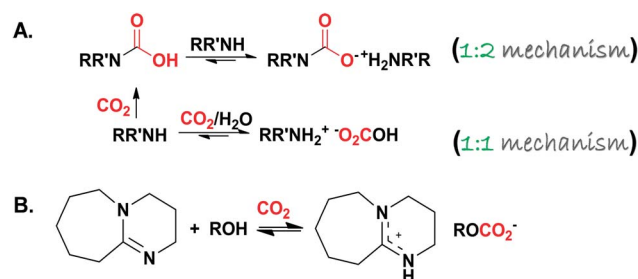
Scheme 3 (A) Proposed chemisorption of CO 2 by amine based substrates (primary and secondary, the general formula is given for the secondary for clarification) through the formation of RR'N-CO 2 - + NH 2 -RR' and RR'NH 2 + + O 2 COH in the absence and presence of water, respectively. (B) The reversible reaction between an alcohol (ROH) and 1,8-diazabicyclo[5.4.0]undec-7-ene (DBU) in the presence of CO 2 .
