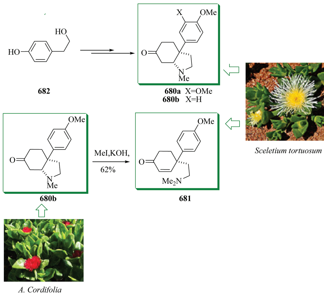
Scheme 147 The formation of 4,5-dihydro-4'-O-methylsceletone 680b into O-methyljoubertiamine 681 .
