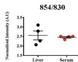
Fig. 4 Calculation of Raman band intensities and intensity ratios pertaining to different biomolecules in liver and serum. Marker bands were chosen for each of the biomolecules; (A) DNA (784 \text{cm}^{-1} ), proteins and lipids (1003, 1451 and 1660 \text{cm}^{-1} ). (B) Ratiometric analysis of two Raman bands – 830 and 854 \text{cm}^{-1} . Each circle in the figure represents an individual mouse. Spectra obtained from a total of 4 mice were used for enumeration. Statistical analysis was performed using Mann–Whitney test where * indicates p < 0.05 .
