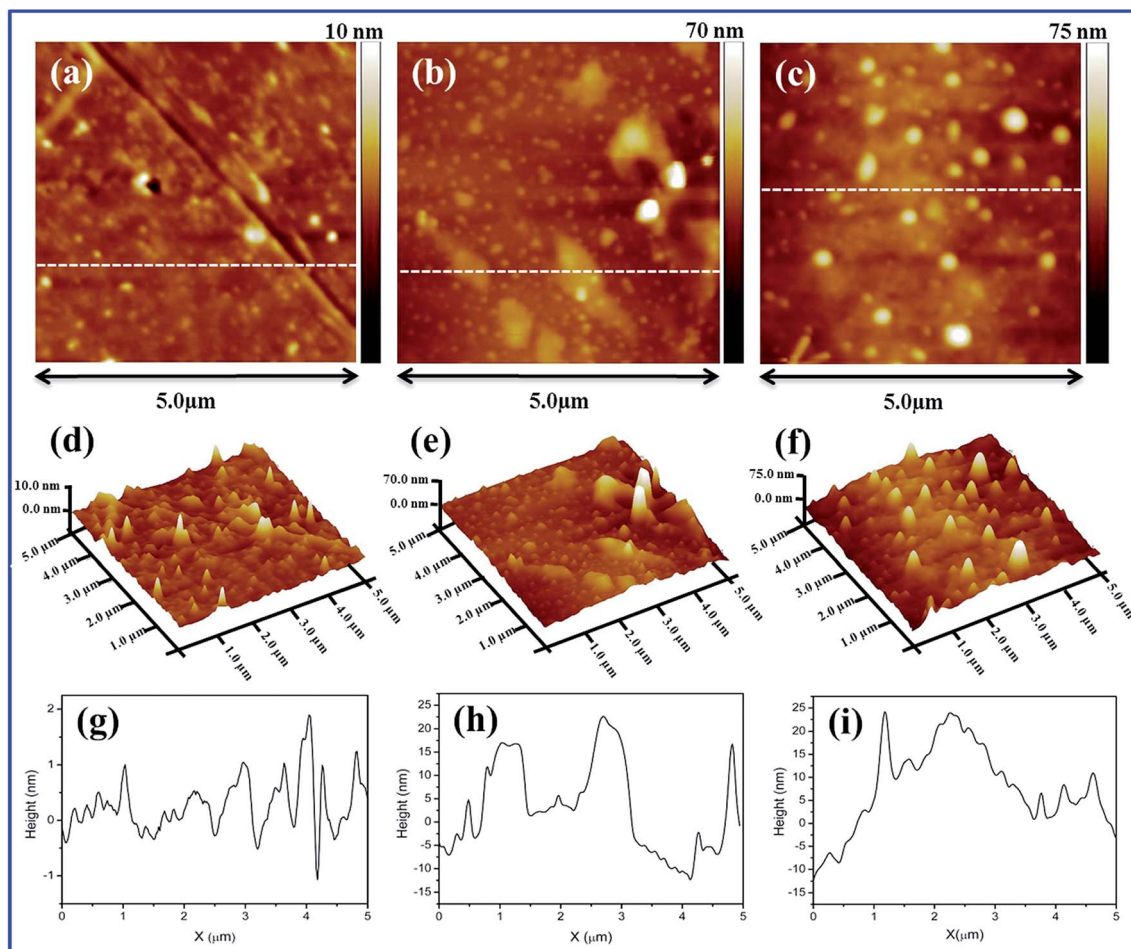
Fig. 5 2D AFM images of membranes of (a) pristine recast Nafion, (b) Nafion/GO-3 and (c) Nafion/SGF-3; 3D AFM images of membranes of (d) pristine recast Nafion, (e) Nafion/GO-3 and (f) Nafion/SGF-3; line profiles of membranes of (g) pristine recast Nafion, (h) Nafion/GO-3 and (i) Nafion/SGF-3.
