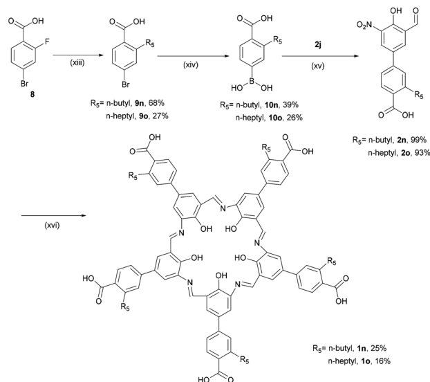
Scheme 3 Syntheses of campestarenes ( 1n and 1o ): (xiii) \text{R}_5\text{MgBr} , \text{THF} , \text{N}_2 , 17 h, then \text{HCl} ; (xiv) n -BuLi, \text{B(O-}i\text{-Pr)}_3 , \text{THF} , -78^\circ\text{C} , 3 h, then \text{HCl} ; (xv) \text{Na}_2\text{CO}_3 , \text{Pd(PPh}_3)_4 , \text{DMF/H}_2\text{O} , 105^\circ\text{C} , 6 h; (xvi) \text{Na}_2\text{S}_2\text{O}_4 , \text{EtOH/H}_2\text{O} , reflux, 2 h.
