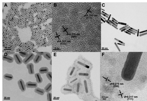
Fig. 1 (A) TEM and (B) HR-TEM images of the synthesized NaGdF 4 :Er 3+ , Yb 3+ UCNP. TEM images of the (C) synthesized GNRs, (D) the SiO 2 coated GNRs (GNR@SiO 2 ), and (E) the hybrid SiO 2 coated GNRs decorated with NaGdF 4 :Er 3+ , Yb 3+ UCNP (GNR@SiO 2 @UCNP), (F) HR-TEM image of the GNR@SiO 2 @UCNP interface.
