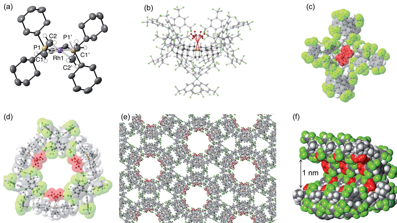
Fig. 2 Solid-state structure of [1-(\text{ethene})_2][\text{BARF}_4]\cdot\text{Hex} with the ethene groups colored in red [(b) to (f)] to highlight their positions. (a) Cation showing the numbering scheme, displacement ellipsoids shown at the 50% probability level; (b) Local environment around the cation showing the arrangement of [\text{BARF}_4]^- anions; (c) Van der Waals radii space-filling representation of (b) showing an alternate view highlighting the \{\text{Rh}(\text{ethene})_2\}^+ fragment; (d) Van der Waals radii space-filling representation showing the packing arrangement leading to a solvent-accessible channel, as viewed down the c -axis; (e) Extended structure viewed down the c -axis; (f) Detail of a channel shown at the van der Waals radii highlighting the arrangement of \{\text{Rh}(\text{ethene})_2\}^+ fragments.
