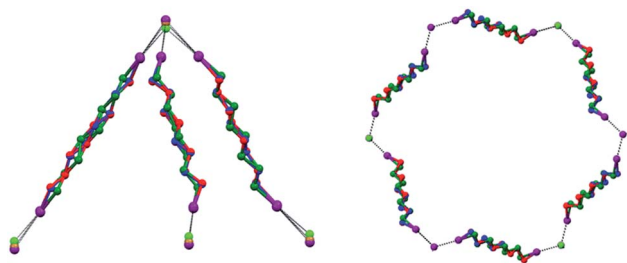
Fig. 7 Left: Superimposition of the trigonal nodes in 1 \cdot 2d \cdot 3d , 1 \cdot 2e \cdot 3d , and 1 \cdot 2f \cdot 3d , evidencing isostructurality. Fluorocarbon chains of modules 3d are green colored in 1 \cdot 2d \cdot 3d cocrystal, blue colored in 1 \cdot 2e \cdot 3d , and red colored in 1 \cdot 2f \cdot 3d , fluorine atoms are omitted; iodide, bromide, and chloride anions are purple, brown, and green, respectively. Right: Superimposition of one hexagonal unit of 1 \cdot 2d \cdot 3d , 1 \cdot 2e \cdot 3d , and 1 \cdot 2f \cdot 3d . XB are black dotted lines. Color codes as left.
