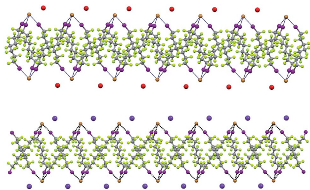
Fig. 8 Representation along the b axis (Mercury 3.8, ball and stick) of one fluororous layer and adjacent cation layers formed by diiodoperfluorooctane 3d with cryptated sodium bromide ( 1 \cdot 2b \cdot 3d , top) or potassium bromide ( 1 \cdot 2e \cdot 3d , bottom). The structural similarity of the pearl necklace (top) and Borromean system (bottom) are apparent. Crypt-222 molecules have been omitted for sake of clarity. Color codes: grey, carbon; green, fluorine; brown, bromine; purple, iodine; red, sodium; violet, potassium.
