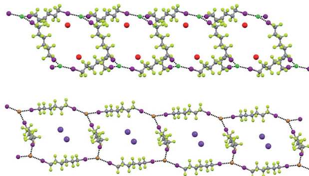
Fig. 9 Representation (Mercury 3.8, ball and stick) of one ribbon of squares formed by diiodoperfluorohexane 3c and cryptated sodium chloride ( 1 \cdot 2a \cdot 3c , top) and potassium bromide ( 1 \cdot 2e \cdot 3c , bottom). Crypt-222 molecules have been omitted for sake of clarity. Color codes: grey, carbon; light green, fluorine; green, chlorine; brown, bromine; purple, iodine; red, sodium; violet, potassium.
