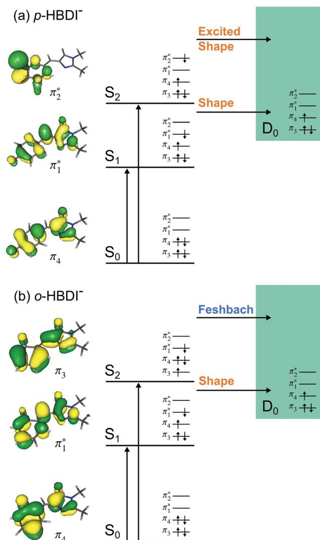
Fig. 6 Energy level diagram of (a) p -HBDI − and (b) o -HBDI − in which possible excitations and subsequent detachment processes are indicated (note that it is only the vibrationally excited states of S 1 lying in the D 0 continuum that have shape resonance character). S 1 and S 2 refer to the first two excited states selected in Table 2. The HOMO is \pi_4 and the LUMO is \pi_1^* . Alongside are the Hartree–Fock molecular orbitals that are involved in the excitations. For op -DHBDI − , a similar scheme applies as for p -HBDI − except the excited state resonance is S 3 (Table 2).
