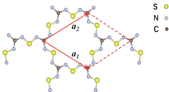
Fig. 1 Schematic representation of the structure of the two-dimensional C_2S_3N_6 monolayer. The unit cell is indicated by the read lines with a_1 and a_2 being the lattice vectors.
