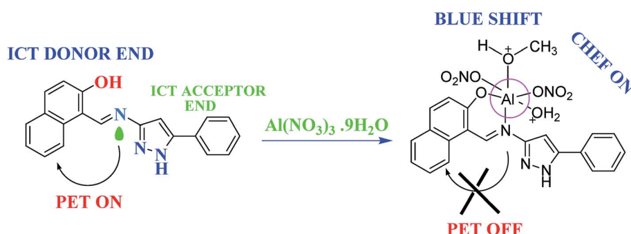
Fig. 8 Probable mechanistic pathway for sensing \text{Al}(\text{III}) ions. 108
