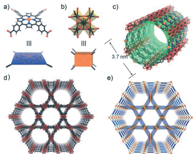
Fig. 1 The crystal structure and underlying network topology of PCN-222(Fe). The Fe- L^1 (a; blue square) is connected to four 8-connected Zr_6 clusters (b; light orange cuboid), generating a 3D network with Kagome-like topology (d, e) and large 1D channels (c; green pillar). Zr: black spheres, C: gray, O: red, N: blue, and Fe: orange. [Reprinted with permission from ref. 56. Copyright 2012, Wiley-VCH Verlag GmbH & Co. KGaA, Weinheim.]
