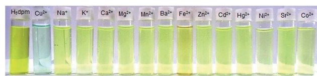
Fig. 2 Visual color change from yellow to sky blue on addition of Cu^{2+} ion in the aqueous solution of H_5dpm among different cations.
