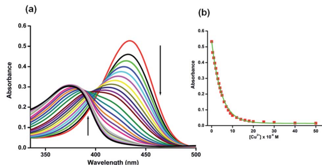
Fig. 1 Left: UV-vis spectra of H_5dpm ( 5 \times 10^{-6} M ) in Tris-buffer solution (25 mM, pH = 7.4) in the presence of various concentration of Cu^{2+} (0, 0.5, 1, 1.5, 2, 2.5, 3, 3.5, 4, 4.5, 5, 6, 7, 8, 9, 10, 12, 14, 16, 18, 20, 25, 30, 40 and 50 ( \times 10^{-6} ) M. Upward arrow indicates gradual increase of absorption at 375 nm wavelength while downward arrow indicates gradual decrease in absorption at 434 nm wavelength with increasing concentration of Cu^{2+} . Right: The absorption of H_5dpm at 434 nm as a function of [Cu^{2+}] in Tris buffer solution (25 mM, pH = 7.4).
