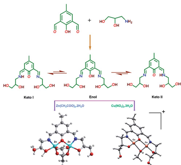
Scheme 1 Synthetic scheme for the synthesis of chemosensor ( H_5dpm ), zinc complex 1 and copper complex 2.
