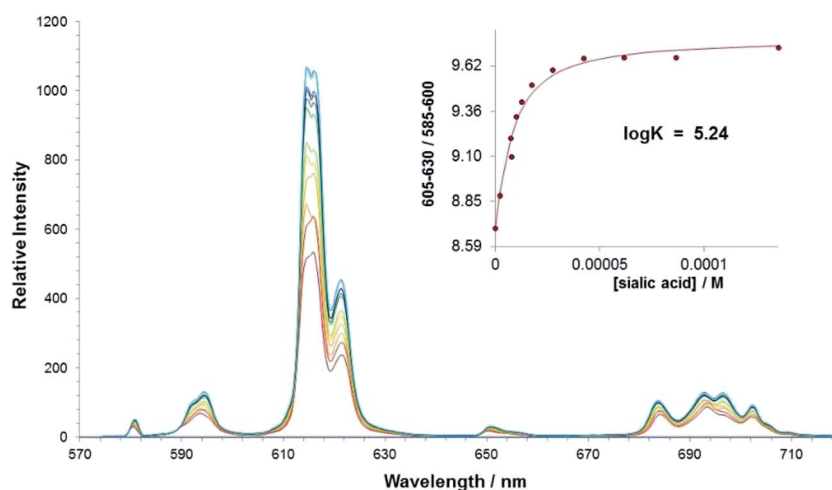
Fig. 5 Variation of the europium(III) emission profile of [Eu·L 1+ ] as a function of added sialic acid. (5 \mu M, \lambda_{exc} = 352 nm, MeOH). Inset shows fit to experimental data, following iterative least squares fitting to a 1 : 1 binding model.
