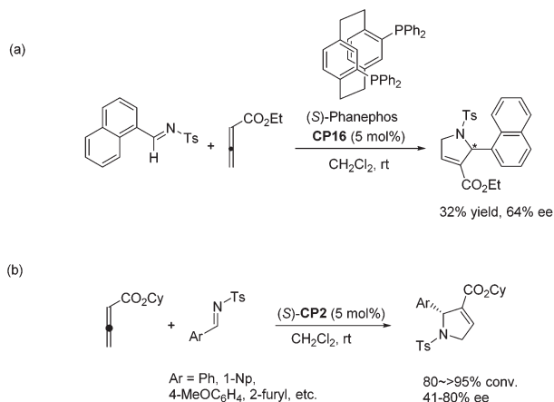
Scheme 27 The catalytic asymmetric Lu's [3 + 2] cycloaddition of allenolates with imines developed by Marinetti's group.
