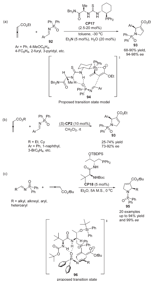
Scheme 28 Enantioselective thiourea-catalyzed [3 + 2] cycloadditions of DPP-imines with allenolates.
