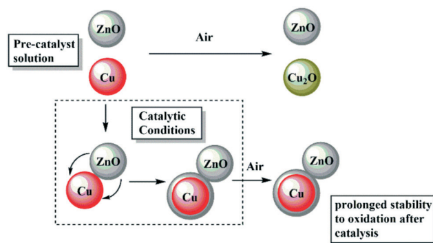
Fig. 7 Schematic illustrating the proposed oxidation of \text{Cu}(0) NPs by air before or after catalysis, with the formation of a Zn containing surface layer during catalysis.
