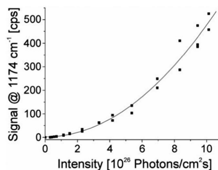
Fig. 3 The square-law dependence of the hyper Raman scattering signal on the excitation intensity verifies the two photon process. The signal of a band at 1174 cm -1 in the SEHRS spectra of 10 -7 M of the dye molecule crystal violet attached to silver nanoaggregates in aqueous solution is shown as a function of the excitation intensity. The spectra were measured using 1064 nm mode locked ps pulses and collection times of 10 seconds. Reproduced with permission from ref. 17. Copyright 2006, National Academy of Sciences, USA.
