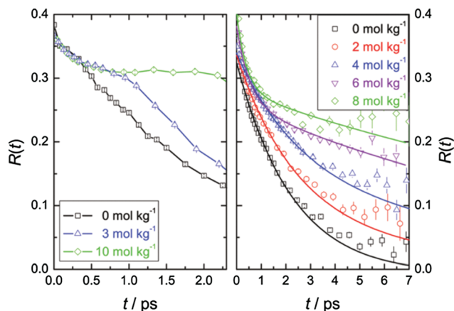
Fig. 3 (left) Anisotropy decay, R(t) , for the O–D vibration of HDO molecules in aqueous TMAO solutions with the pump pulse centered at around 2440\text{ cm}^{-1} for various TMAO concentrations. (right) R(t) with the pump pulse centered at around 2560\text{ cm}^{-1} . Figures are adapted from ref. 5 with permission of the American Chemical Society.
