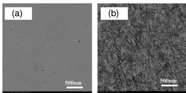
Fig. 20 Transmission electron microscopy images of the (a) P3HT/F8BT blend film prepared from DCB and (b) P3HT-nanowire/F8BT blend film prepared from a mixed solution of DCB and n -hexane. The scale bar corresponds to a length of 500 nm. All the blend films have a thickness of ~80 nm. Reproduced with permission from (ref. 53). Copyright 2014, American Chemical Society.
