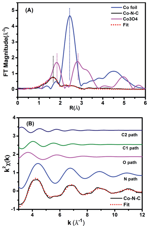
Fig. 3 (A) The k^2 -weighted Fourier transform spectra of the experimental and fitted Co-N-C catalyst as well as the Co foil and Co 3 O 4 reference samples. (B) The contributions of different paths including Co-N (blue line), Co-O (pink line) and Co-C (green and navy blue lines) in k -space for the Co-N-C sample.
