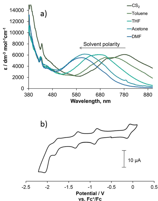
Fig. 1 (a) UV/vis absorption spectra of complex 3 recorded in solvents of different polarity and (b) the cyclic voltammogram of 3 in DMF with [\text{t}^{\text{Bu}}_4\text{N}][\text{BF}_4] (0.2 M) as supporting electrolyte at a scan rate of 0.1 \text{ V s}^{-1} .
