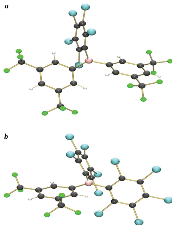
Fig. 2 (a) X-ray crystallographic structure of \text{B}\{3,5-(\text{CF}_3)_2\text{C}_6\text{H}_3\}_2(\text{C}_6\text{Cl}_5) 5. (b) X-ray crystallographic structure of \text{B}(\text{C}_6\text{Cl}_5)_2\{3,5-(\text{CF}_3)_2\text{C}_6\text{H}_3\} 6 (minor component of crystallographic disorder removed for clarity).
