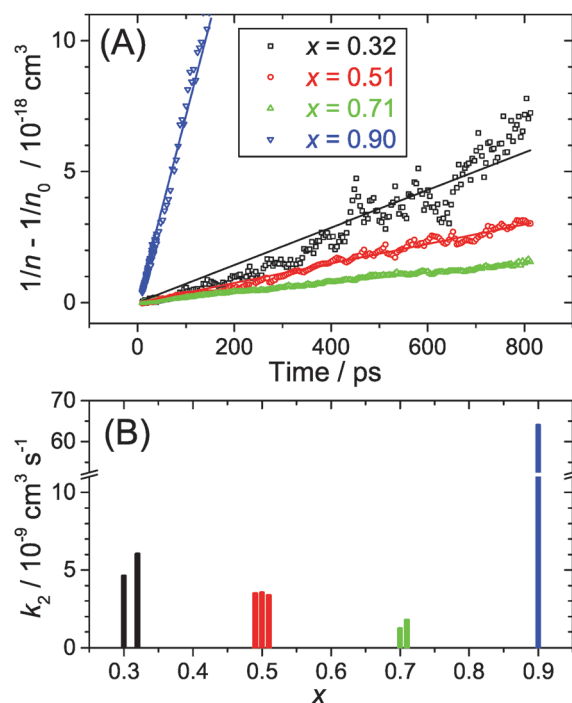
Fig. 8 (A) Plot of the difference of the reciprocal transient ( n ) and initial ( n_0 ) carrier density as a function of time for the (\text{MAI})_x(\text{PbI}_{2-x})/\text{TiO}_2/\text{glass} samples employing MAI mole fractions x = 0.32 (black), 0.51 (red), 0.71 (green) and 0.90 (blue). The slope corresponds to the second-order rate constant k_2 for electron-hole recombination, which is more than one order of magnitude larger for low-dimensional perovskites ( x = 0.90 ). The data and fits in the plots are for high pump fluence ( 50 \mu\text{J cm}^{-2} ). (B) Plot of the second-order rate constant k_2 as a function of the MAI mole fraction x for multiple determinations. Note the break on the k_2 axis.
