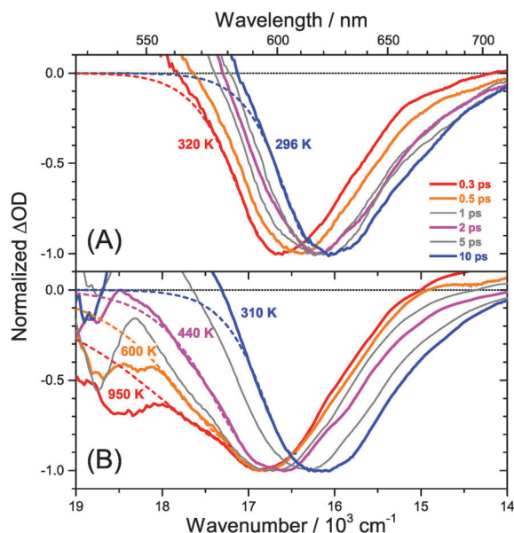
Fig. 7 Normalized transient PSCP broadband absorption spectra of (\text{MAI})_x(\text{PbI}_{2-x})/\text{TiO}_2/\text{glass} ( x = 0.90 ) for (A) 2 \mu\text{J cm}^{-2} pump fluence and (B) 50 \mu\text{J cm}^{-2} pump fluence. (red) 0.3 ps, (orange) 0.5 ps, (grey) 1 ps, (magenta) 2 ps, (grey) 5 ps and (blue) 10 ps. Dashed coloured lines represent fits to the Boltzmann tail of the carrier distribution by the procedure described in the text, resulting in the carrier quasi-temperatures provided in the figure. For higher pump fluences, carrier cooling is substantially slower.
