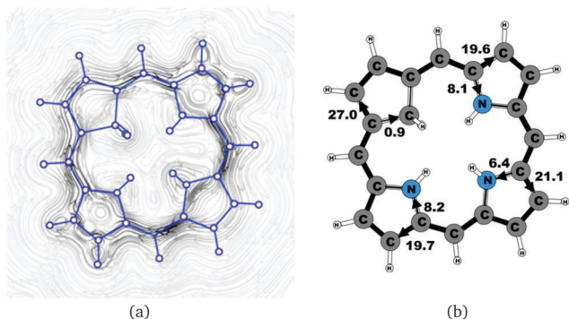
Fig. 3 (a) A streamline plot of the current density 1 bohr above the carbaporphyrin 20H 2 2+ molecule that sustains a net ring-current strength of 27.8 \text{ nA T}^{-1} around the porphyrinoid macroring. (b) The calculated net current strengths (in \text{nA T}^{-1} ) passing selected bonds are given for carbaporphyrin 20H 2 2+ .
