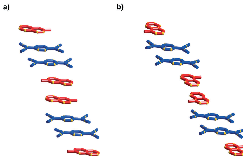
Fig. 1 Representations of a) (1)(TCNQ) and b) (2)(TCNQ) viewed almost normal to the stacking direction. The cation is indicated in red and the TCNQ •- in blue.
