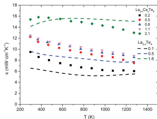
Fig. 9 Thermal conductivity as a function of temperature for \text{La}_{3-x}\text{Ca}_x\text{Te}_4 as compared to \text{La}_{3-x}\text{Te}_4 . 7
