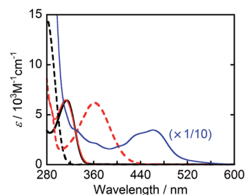
Fig. 1 UV-vis absorption spectra of \text{BIH} (black solid line), \text{BI}^+ (black broken line), \text{BI(OH)H} (red solid line), \text{BI(O}^{\ominus}\text{)}^+ (red broken line), and \text{Ru}_2\text{-Ru(CO)} (blue line, 1/10 intensity) in DMF-TEOA (4 : 1 v/v).
