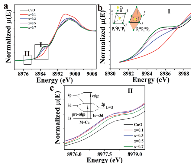
Fig. 3 (a) Normalized Cu–K edge XANES spectra for \text{Cu}_x\text{Ir}_{1-x}\text{O}_6 compositions. (b) Shows the shakedown transition and the inset is a diagram of the Cu-4p orbital energy in two different symmetries. (c) Shows the amplified pre-edge region and the inset diagram shows the energy level of possible transitions. (b) and (c) correspond to the selected areas, I and II, in (a).
