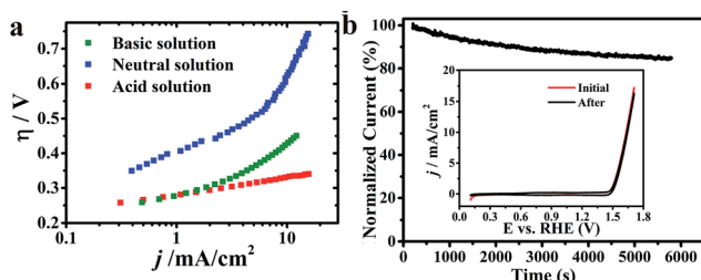
Fig. 1 OER activity of \text{Cu}_{0.3}\text{Ir}_{0.7}\text{O}_6 in three solutions of different pH. (a) Tafel curves of \text{Cu}_{0.3}\text{Ir}_{0.7}\text{O}_6 . The R in the three solutions was \sim 18\ \Omega (acid), \sim 15\ \Omega (neutral) and \sim 28\ \Omega (basic), respectively. (b) Chronoamperometric curves at the constant potential 1.68 V vs. RHE. The insert shows the polarization curves for \text{Cu}_{0.3}\text{Ir}_{0.7}\text{O}_6 at the initial time point and after the chronoamperometric experiments. The catalyst loadings were 0.2\ \text{mg cm}^{-2} on a Ti plate.
