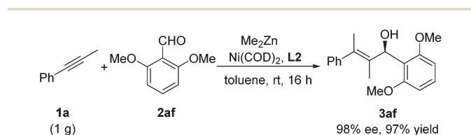
Scheme 1 Gram-scale asymmetric alkylative alkyne–aldehyde cross-coupling.
