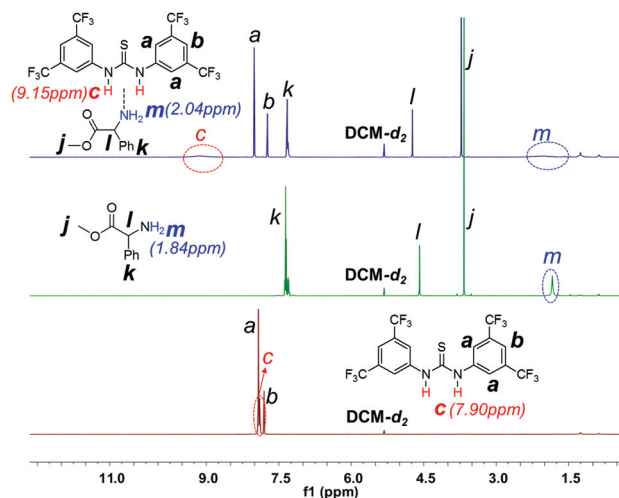
Fig. 7 ^1\text{H} NMR spectra of TU-S, methyl 2-amino-2-phenylacetate (MAP) and TU-S/MAP mixture (500 M, 25 \text{ }^\circ\text{C} , \text{CD}_2\text{Cl}_2 , for full spectrum of the mixture see Fig. S13†).
