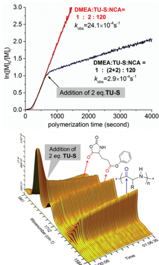
Fig. 6 \ln([\text{NCA}]_0/[\text{NCA}]_t) vs. time for the ROP of Glu-NCA initiated by DMEA/TU-S ( [\text{M}] = 0.19 \text{ M} , [\text{Glu-NCA}]/[\text{TU-S}]/[\text{DMEA}] = 120/(2 + 2)/1 , 25 \text{ }^\circ\text{C} , \text{CH}_2\text{Cl}_2 ) and corresponding 3D kinetic behavior profile from in situ IR (the sampling interval of in situ IR is 10 seconds).
