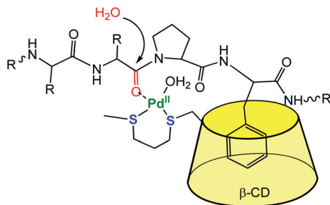
Bradykinine sequence: Arg-Pro-Pro-Gly-Phe-Ser6-Pro7-Phe-Arg
