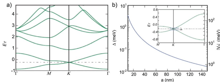
Fig. 19 (a) AG Minibands (energy is in meV) with a lattice period a = 60 nm, r_0 = 0.2a ( r_0 is the width of the potential well) and V_0 = 5 meV. A dashed-dotted line is drawn at the Dirac-point energy. (b) Energy width, \Delta , of the linear part of the spectrum near the Dirac point as a function of a . V_0 is varied correspondingly (see the right vertical axis) in order to obtain an isolated Dirac point, i.e. without any other state inside the bulk BZ at the Dirac-point energy. Inset: magnification of the energy bands in panel (a) around the Dirac point energy. The blue dashed lines mark the energy limits of the linear dispersion approximation. Adapted from ref. 260.
