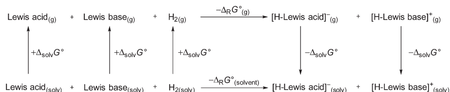
Fig. 2 Born-Haber-Fajans cycle to access the \Delta_r G^\circ_{(g)} and \Delta_r G^\circ_{(\text{solv})} of 1 and \text{B}(\text{C}_6\text{F}_5)_3 in various solvents.
