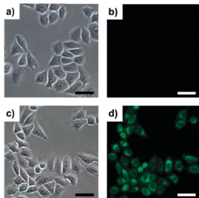
Fig. 30 Top: reaction of dicyanoethylene BODIPY 36 with \text{CN}^- . Bottom: brightfield (a, c) and fluorescence (b, d) images of HeLa cells with only 36 (a, b) then 20 min after treatment with NaCN (c, d). Scale = 50 \mu\text{m} . Image reproduced with permission. 176
