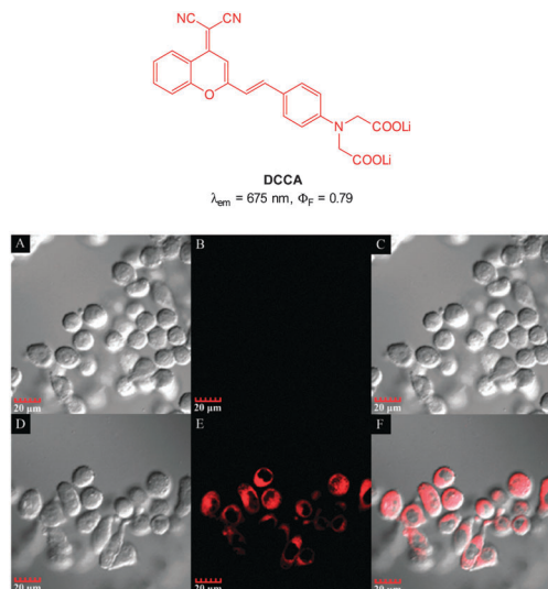
Fig. 41 Top: structure of copper ligand DCCA . Bottom: confocal fluorescence images in KB cells: (A–C) cells incubated with DCCA 2 -Cu(II) alone. (D–F) Cells incubated with DCCA 2 -Cu(II), then K 4 P 2 O 7 . Emission collected at 630–730 nm, excitation at 405 nm. Bright field (A and D), fluorescence (B and E) and overlap field (C and F). Image reproduced with permission. 192
