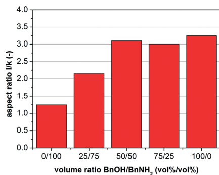
Fig. 3 Influence of the solvent on the morphology of the AZO nanocrystals.
