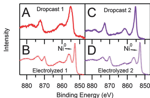
Fig. 4 High resolution XPS spectra of the Ni 2p region. (A) Dropcast 1 onto gold plated silica wafer. (B) Electrolyzed 1 on a glassy carbon plate from a 0.38 mM 1 and 13.6 eq. CF 3 COOH solution. (C) Dropcast 2 onto gold plated silica wafer. (D) Electrolyzed 2 on a glassy carbon plate from a 0.38 mM 2 and 13.6 eq. CF 3 COOH solution. Electrolyzed solutions contained 0.1 M [Bu 4 N][PF 6 ] and were held at −1.66 V vs. Fc + /Fc for 480 s.
