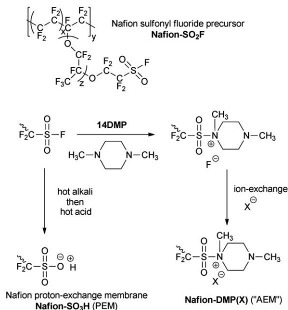
Scheme 1 The proposed reaction of Nafion® sulfonyl precursor [Nafion-SO 2 F] with 1,4-dimethylpiperazine [14DMP] to form an AEM in X – anion form [Nafion-DMP(X)]. Also shown is the process to generate the standard PEM form of Nafion® [Nafion-SO 3 H]. X = anion being studied.
