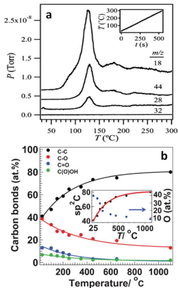
Fig. 14 (a) Temperature programmed desorption spectra of GO film thermally reduced at heating rate of 30\text{ }^{\circ}\text{C min}^{-1} ; m/z = 18, 44, 28, 32 indicate \text{H}_2\text{O} , \text{CO}_2 , CO, and \text{O}_2 , respectively. The inset is the heating rate curve. Reprinted with permission from ref. 188. Copyright (2009) American Chemical Society. (b) The atomic percentage of different carbon atoms identified by XPS with respect to the annealing temperatures. The inset indicates the oxygen percentage evolution during the reduction process. Reprinted with permission from ref. 106. Copyright (2009) John Wiley and Sons.
