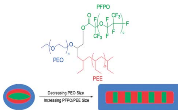
Fig. 3 The transition in morphology in aqueous solution of an ABC-type miktoarm star, from “hamburger” micelles (left) to segmented worms (right), as hydrophobicity of the polymer increases. The colors in the picture of the self-assembled structures (bottom) correspond to the polymer’s structure (above).
