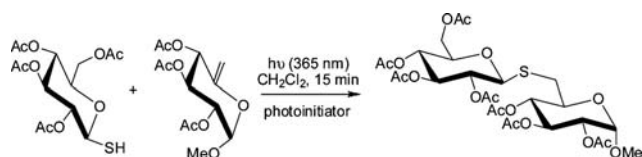
Scheme 32 Radical-induced thiol-ene coupling between a peracetylated glucosylthiol and a hex-5-ene-2-pyranoside under photochemical conditions.
