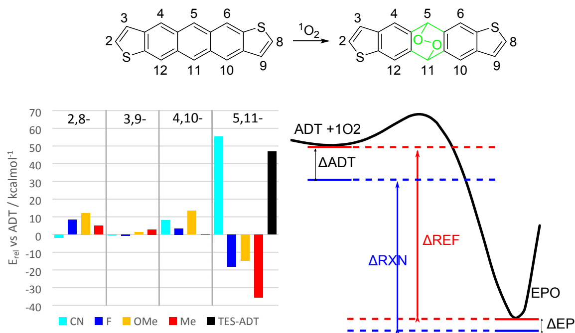
Figure 8. (Left) Computed reaction enthalpies for endoperoxide formation from difunctionalised ADT derivatives with substituents in varying position around the acene periphery. All energies relative to unsubstituted ADT, where positive values indicate greater stability. Green atoms in the chemical structure denote those which are not part of the conjugated \pi -system. (Right) Reaction path diagram indicating how relative stabilisation of ADT and EPO (black arrows) affects the overall reaction enthalpy (red and blue arrows).
