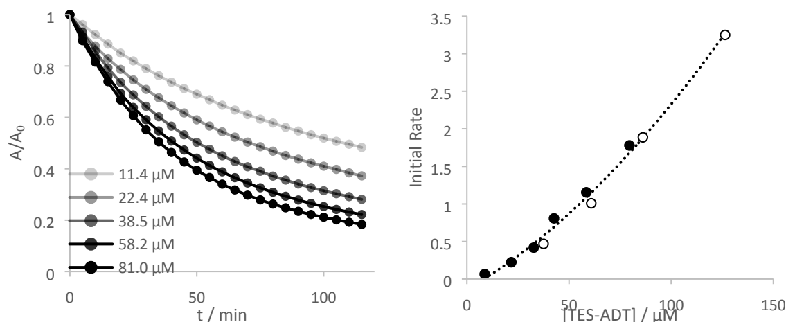
Figure 4. Normalised absorption at 555 nm over time of solutions of TES-ADT in \text{CHCl}_3 at different concentrations (darker = more concentrated) under illumination by green LED. (right) plot of initial rate versus initial concentration. Filled circles monitored the first vibronic peak (555 nm) while the open circles were from a repeat experiment using the second vibronic peak (515 nm) allowing higher concentrations without saturating the detector.
