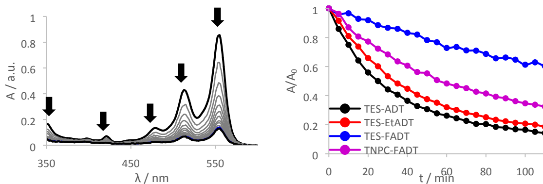
Figure 2. (Left) Absorption spectra of TES-ADT in CHCl 3 measured at timed intervals while under illumination from an LED desk lamp. (Right) Normalised absorbance at \lambda_{\max} for ADTs over time, while under illumination from an LED desk lamp.
