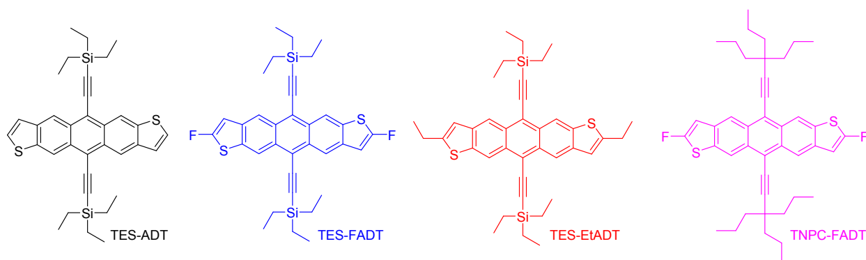
Figure 1. Chemical structures of anthradithiophene derivatives in our initial investigation.
