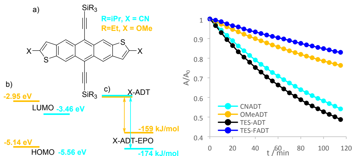
Figure 7. a) Structure of TES-OMeADT (orange) and TIPS-CNADT (cyan), b) molecular orbital energies estimated from cyclic voltammetry, c) computed reaction enthalpies for endoperoxide formation, d) normalised absorbance of TIPS-CNADT and TES-OMeADT in \text{CHCl}_3 at 33 \mu\text{M} under irradiation by white LED. TES-ADT and TES-FADT (same conditions) are shown for comparison.
