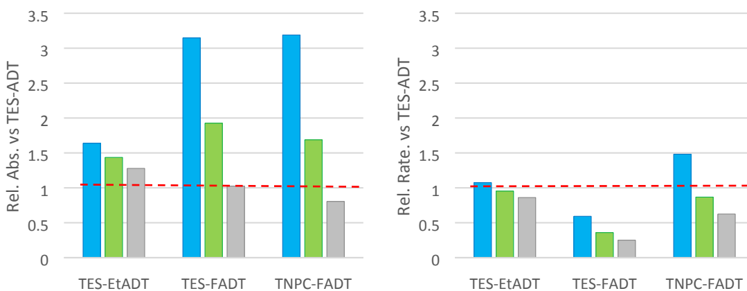
Figure 3. (Left) Integrated absorbance of ADTs versus light source spectra relative to the parent TES-ADT. (Right) Relative reaction rates for photo-oxidation of ADTs using different coloured light sources, estimated from linear fits of absorbance over 10 minutes where A/A_0 > 0.9 . All data relative to values determined for parent TES-ADT (depicted as the red line) with the same light source (blue, green, or white LED) and same concentration ( 3.3 \mu\text{M} in \text{CHCl}_3 ).
