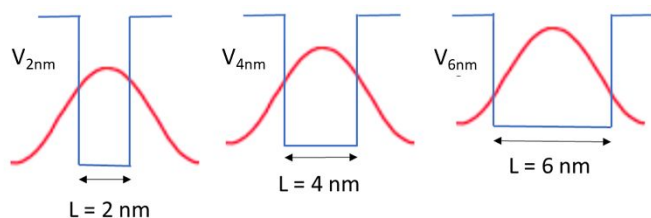
Figure 7. Schematic of proposed mechanism of how wavefunction overlap in a PIB model differs with NP size in small (L=2), medium (L=4), and large (L=6) size regimes. The rectangles shown represent the comparative size of the boxes for each NP size. The red curve represents a simple n=1 wavefunction for the NP exciton if it were not confined. V_{2nm} , V_{4nm} , and V_{6nm} represent the height of the boxes or the potential barriers, and are dependent on the ionization potentials of the respectively sized NPs.
