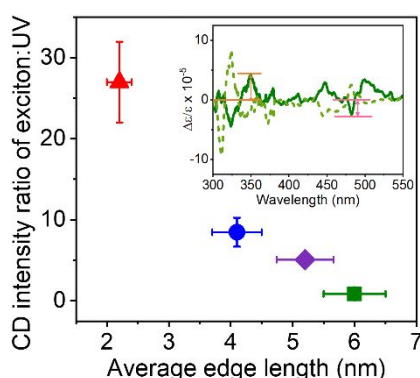
Figure 5. Plot of the ratio of the exciton:UV region CD intensity versus the NP edge length for 2nm (red), 4nm (blue), 5nm (purple), and 6nm (green) NPs. Inset shows a representative CD spectrum with the UV and the exciton intensity marked in orange and pink respectively.
