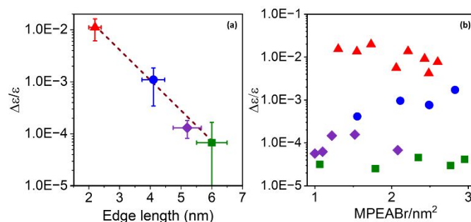
Figure 4. (a) Average CD intensity plotted on a logarithmic scale as a function of average edge length for a chiral NP in the 2nm (red), 4nm (blue), 5nm (purple), and 6nm (green) size regimes. The brown dotted line shows a line of best fit, with a slope of -1.35 \text{ nm}^{-1} . (b) CD intensity plotted on a logarithmic scale as a function of chiral ligand (MPEABr) coverage for the different NP sizes
