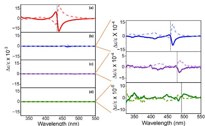
Figure 3. Circular dichroism (CD) spectra for (a) 2nm, (b) 4nm, (c) 5nm, and (d) 6nm NPs in toluene are shown. Orange lines indicate zoomed in spectra of the 4nm, 5nm (x10), and 6nm (x100) NPs shown in panels to the right. Chiral NPs with R-MPEABr and S-MPEABr on the surface are shown using solid and dotted lines respectively. The wavelength for the first excitonic transition is marked by black dotted line in each spectrum.
