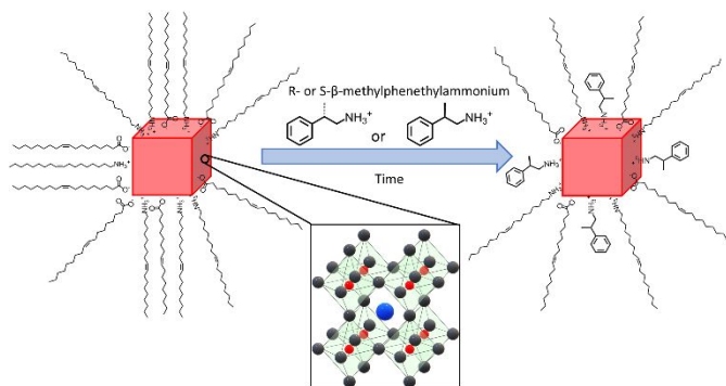
Figure 1. Schematic of post-synthetic ligand exchange on CsPbBr 3 NPs (represented by red cubes). The insert depicts the crystal structure of the NPs where the Pb 2+ (red) and Br - (black) ions arranged in corner-sharing octahedra, with Cs + ions (blue) surrounded by the PbBr 6 4- octahedra. The achiral NP shown on the left is capped by oleic acid and oleylamine, while after ligand exchange, some of the native achiral ligands are replaced by R/S-methylphenethylammonium ligands (as shown on the right).
