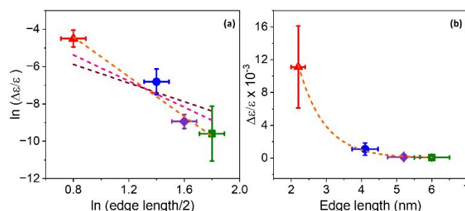
Figure 6. (a) The natural log of average CD intensity plotted as a function of the natural log of half of the average edge length for a chiral NP in the 2nm (red), 4nm (blue), 5nm (purple), and 6nm (green) size regimes. The brown dashed line shows a line of best fit with a slope fixed at -2 , the pink dashed line shows a line of best fit with a slope fixed at -3 , while the orange dashed line shows a line of best fit where the slope is allowed to float, which gives a best fit slope of -5.3 . (b) Average CD intensity vs NP edge length fitted to an exponential decay law of y=ae^{-bx} , where a = 0.22 and b = 1.35 , with an adjusted R^2 fit of 0.98 .
